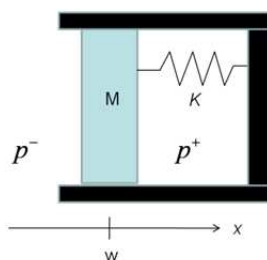
Figure 1: Schematic representation of the analytical model.
