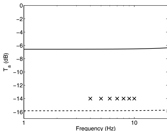
Figure 5: Magnitude of the transmission coefficient: experimental results (cross), analytical predictions with pinned plate assumption (solid line) and clamped plate assumption (dashed line).
