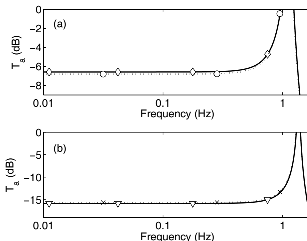
Figure 4: Magnitude of the transmission coefficient simulated by FEM and analytical model for two load cases: (top) pinned plate and (bottom) clamped plate. (circle marker) analytical pinned plate, (diamond) FEM pinned plate, (triangle) analytical clamped plate, (cross) FEM clamped plate.
