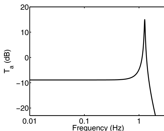
Figure 2: Magnitude of the transmission coefficient.
