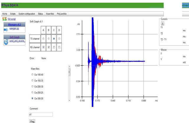
Figure 6: Screenshot of the IO interface. Left, operator friendly build the desired E-R configuration and choose a signal for emission. Right, plot of the received signals on both channels.
