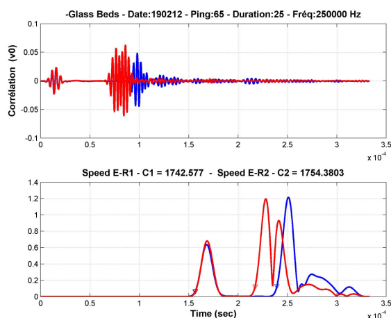
Figure 9: Sound speed processing for a ping at 250kHz in glass beads. Top, voltage versus time of received signals (in blue for channel 1, in red for channel 2). Bottom, envelop of the correlated signal showing emitted and received signal spikes used for time of flight calculation.
