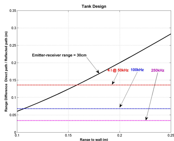
Figure 1: Size constraints for the tank. We report the range difference RD between direct and wall-reflected path versus the range to the side wall (in black).
