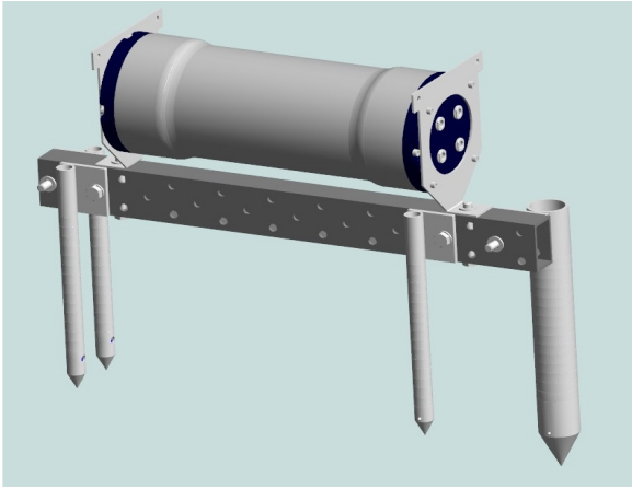
Figure 5: Drawing of the celerimeter prototype.
