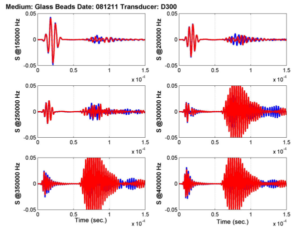
Figure 7: From top left to bottom right, received signals at 150, 200, 250, 300, 350, 400 kHz (channel 1 in red, channel 2 in blue). Note that amplitude scale is the same for all captions (there is no saturation on the three last signals).
