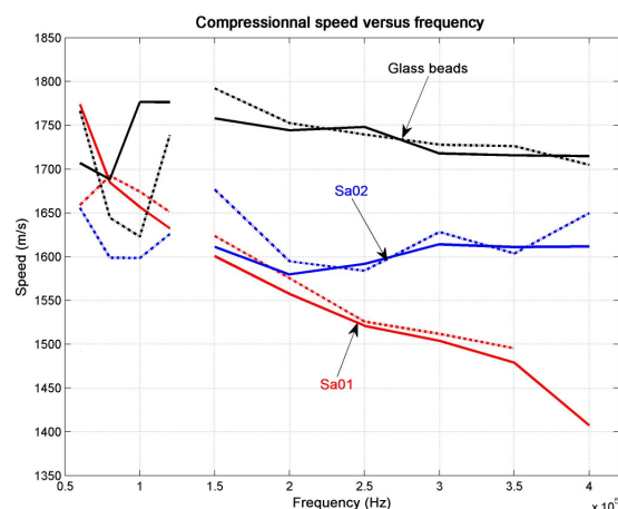
Figure 10: Sound speed versus frequency for the three samples, between 60kHz and 400kHz (dashed lines for channel 1). Results enclose SP1 and SP2 transducer contributions.
