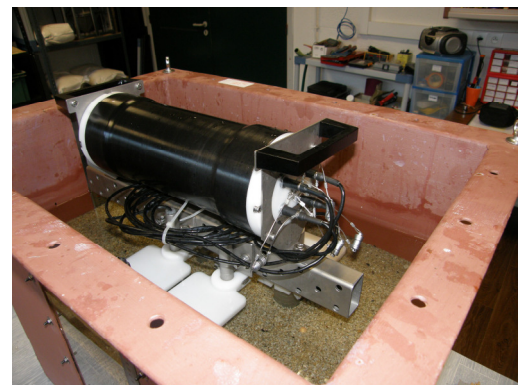
Figure 8: Celerimeter measuring Sa02 sound speed in tank.
