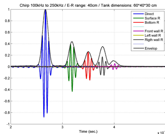
Figure 2: simulation of the multipath inside the tank.
