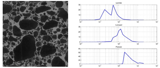
Figure 4: Left, image of the sand Sa02. Right, three stored marine sands with very different granulometry (from top to bottom, Sa01, Sa02 and Sa03).
