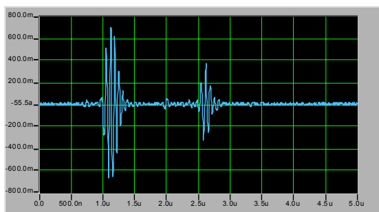
Figure 3: Example of ultrasonic signal backscattered by a sample of the Navel orange.
