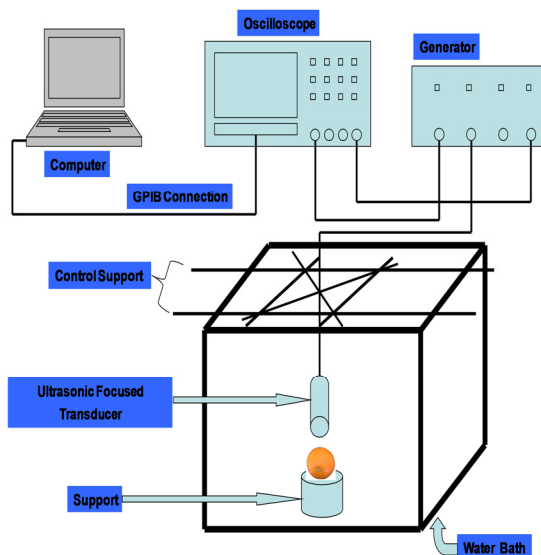
Figure 2: Diagram of the ultrasonic measuring system.
