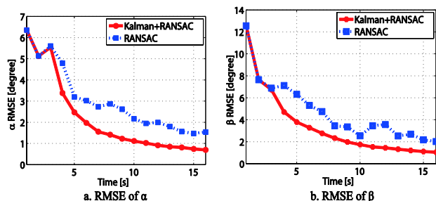
Figure 4: The RMSE of direction angles in a dynamic tracking situation. (Dotted square line: RANSAC; Solid point line: RANSAC + Kalman)
