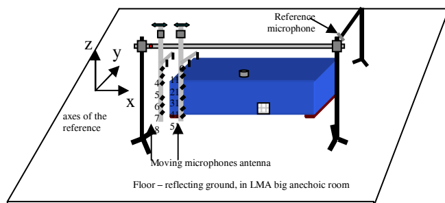
Figure 2: measurement set-up
