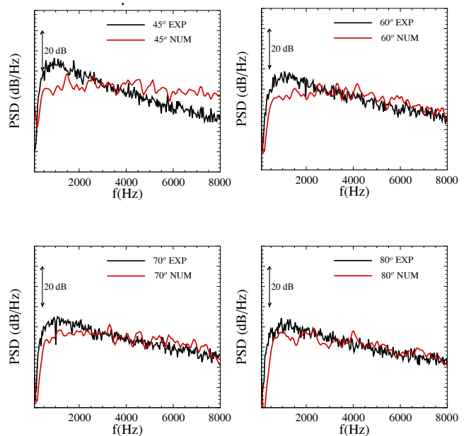
Figure 8: Power spectral density of the pressure signals for different observers located at r = 10D from the nozzle exit.
