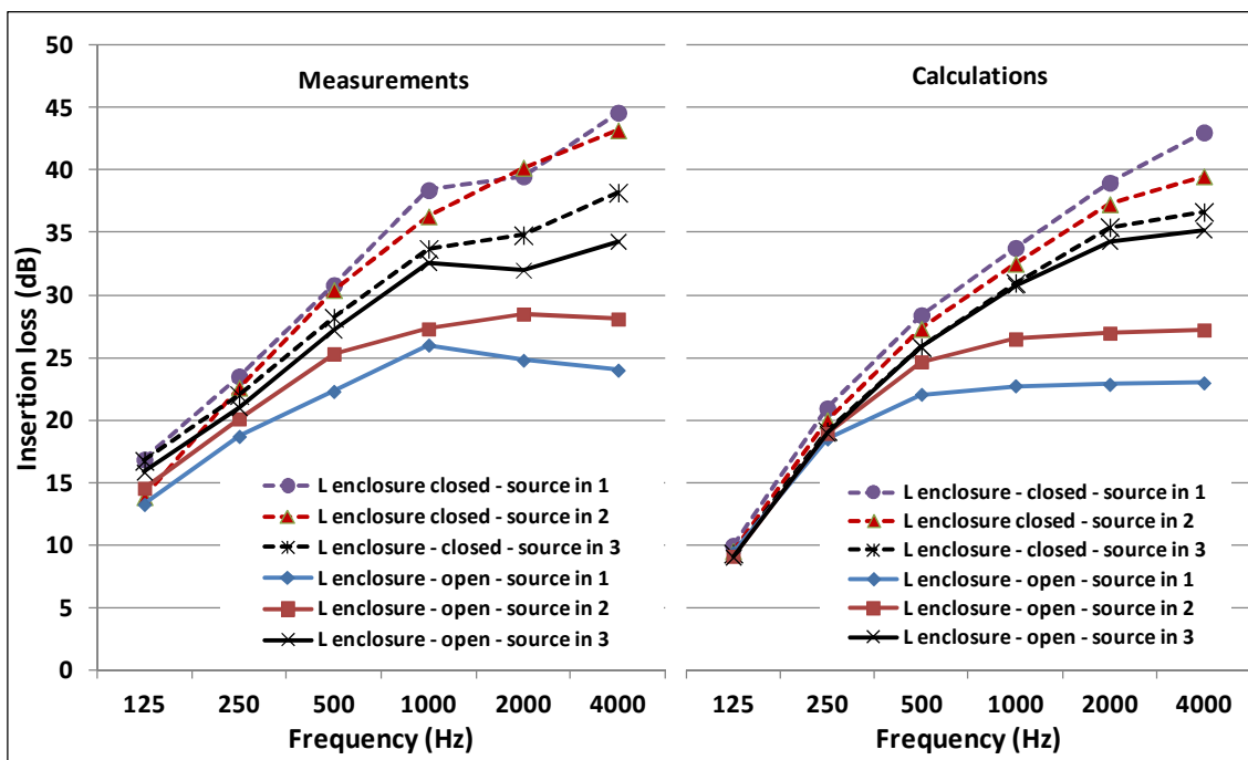
Figure 2: Insertion loss of the L-shaped single-leaf enclosure for various configurations – comparisons between measurements and calculations
