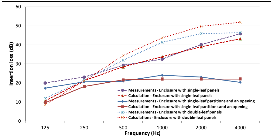
Figure 1: Insertion loss of rectangular enclosures – comparisons between measurements and calculations
