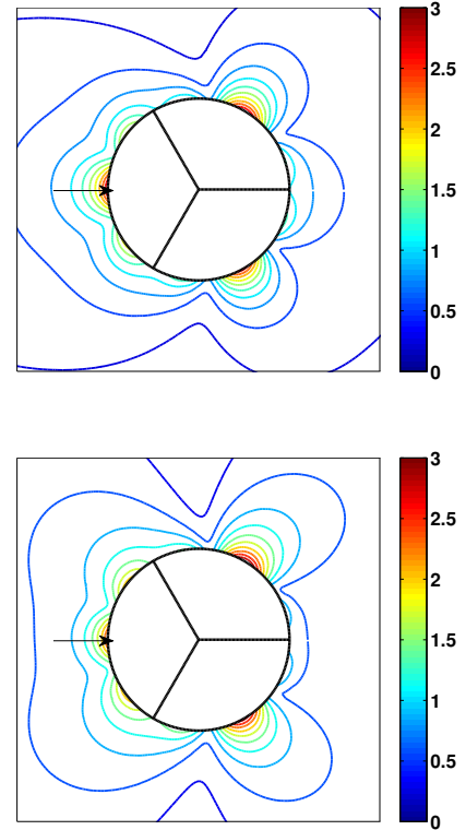
Figure 4: Pressure field in the external fluid at f = 100 Hz for an incompressible (top) and compressible (bottom) hypothesis for the external fluid.
