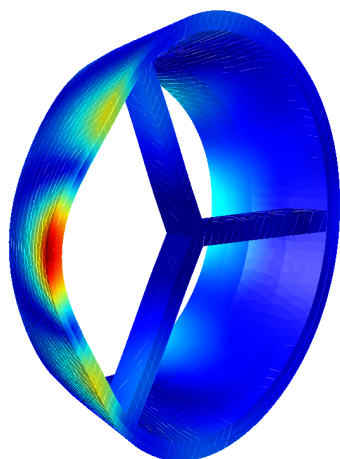
Figure 11: Deformed shape of the structure at 197 Hz.
