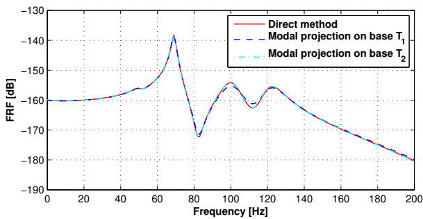
Figure 5: Frequency response of the damped structure by a direct method, a modal projection of Eq.8 on basis
