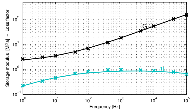
Figure 2: Master curves of Deltane 350 at 12°C (crosses : experimental datas, line : fitted results)
