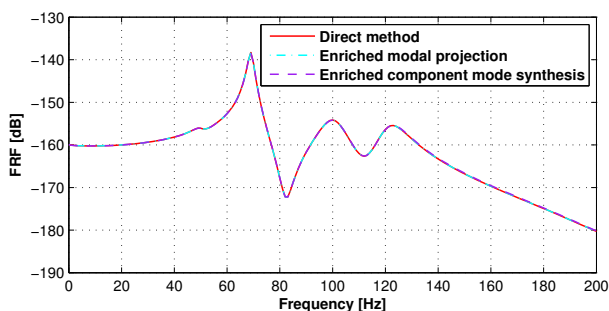
Figure 8: Frequency response of the damped structure by a direct method, a modal projection of Eq.8 on basis \mathbf{T}_2 = [\phi_{1..24}, \psi_{1..24}(f_c = 200\text{Hz}), \mathbf{T}_S] and an enriched component mode synthesis applied to the substructuring described on Figure 6 with 12 real undamped fixed-interface modes and 12 fixed-interface modes calculated with a shear modulus evaluated at the frequency f_c = 200\text{Hz} per component.
