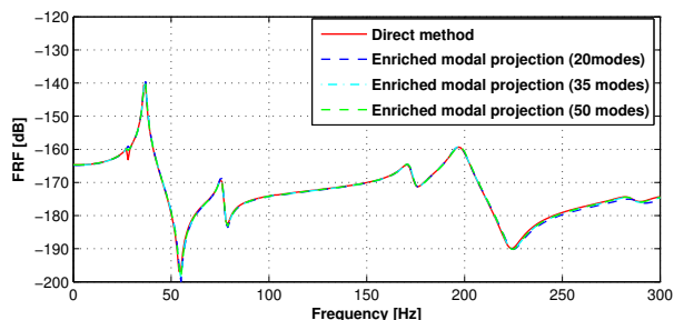
Figure 10: Frequency response function of the structure calculated from a direct method and an enriched modal projection using 20, 35 and 50 modes \phi_i and \psi_i .
