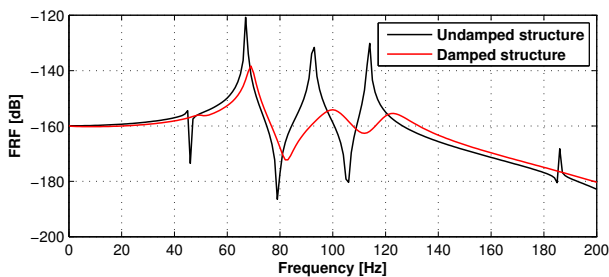
Figure 3: Direct frequency response of the structure
