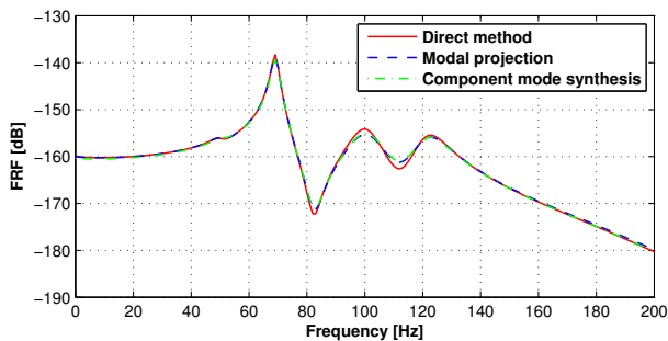
Figure 7: Frequency response of the damped structure by a direct method, a modal projection of Eq.8 on basis \mathbf{T}_1 = [\phi_{1..48}, \mathbf{T}_S] and a component mode synthesis applied to the substructuring described on Figure 6 with 24 modes per component.
