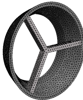
Figure 9: Tridimensional structure studied.
