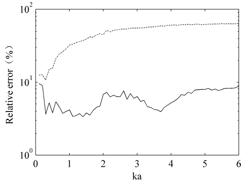
Figure 4: The relative errors between the theoretical free-field pressure and the outgoing pressure (dotted line), and those between the theoretical free-field pressure and the recovered free-field pressure (solid line).
