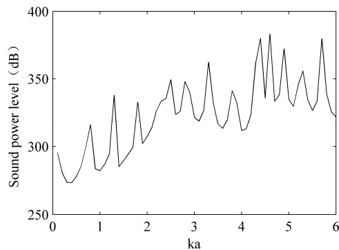
Figure 8: Sound power level on the surface S_1 .
