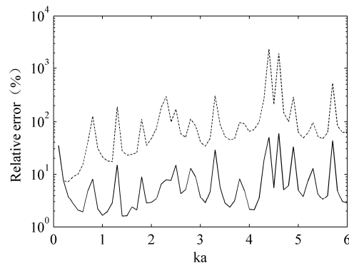
Figure 7: The relative errors between the theoretical free-field pressure and the outgoing pressure (dotted line), and those between the theoretical free-field pressure and the recovered free-field pressure (solid line).
