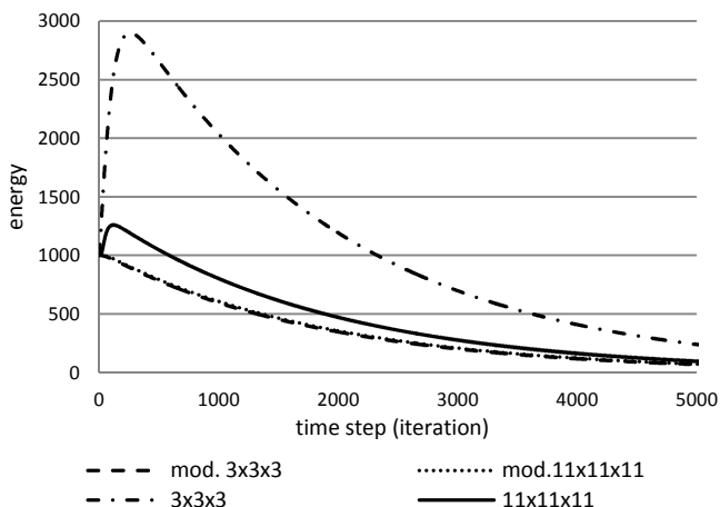
Figure 5: Energy decays for cubic room 10x10x10m built from 3x3x3pts, and 11x11x11 pts, modelled using modified and unmodified equations; \Delta t=0,0001s .
