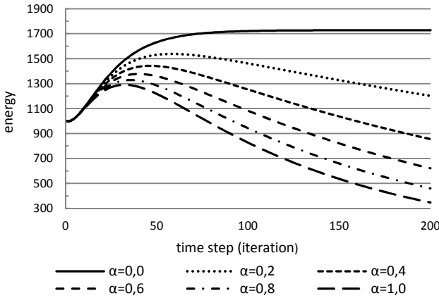
Figure 3: Energy distribution in 6 x 6 x 6 pts model as a function of absorption coefficient, for values: \Delta x=1\text{m} , \Delta t=0,0001\text{s} .
