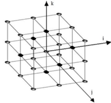
Figure 1: Schematic draw of calculation nodes net. With darker color are marked nodes on the basis of the energy of node placed in the centre is calculated.
