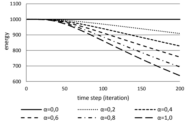
Figure 4: Energy distribution in 6 x 6 x 6 pts model as a function of absorption coefficient, for values: \Delta x=1\text{m} , \Delta t=0,0001\text{s} , after modification.
