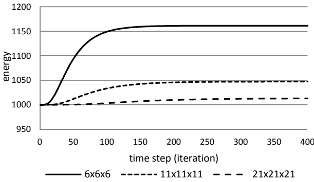
Figure 2: Energy distribution in 3D model as a function of model size for values: \alpha=0 , \Delta x=1\text{m} , \Delta t=0,0001\text{s} .
