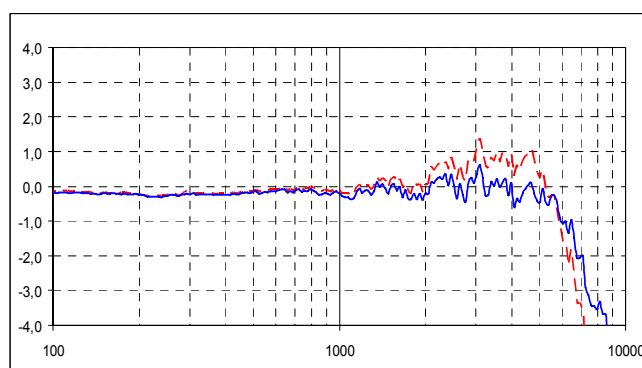
Fig. 10: corresponding frequency response
