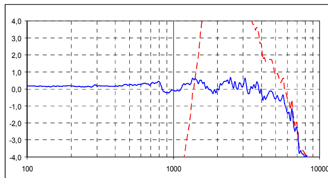
Fig. 6: corresponding frequency response
