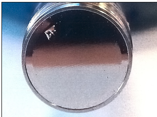
Fig. 1: microphone with damaged membrane
