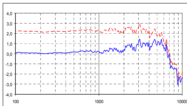
Fig. 18: corresponding frequency response
