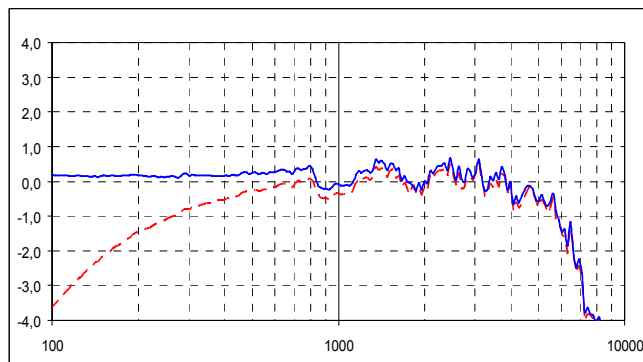
Fig. 20: corresponding frequency response
