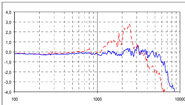
Fig. 12: corresponding frequency response
