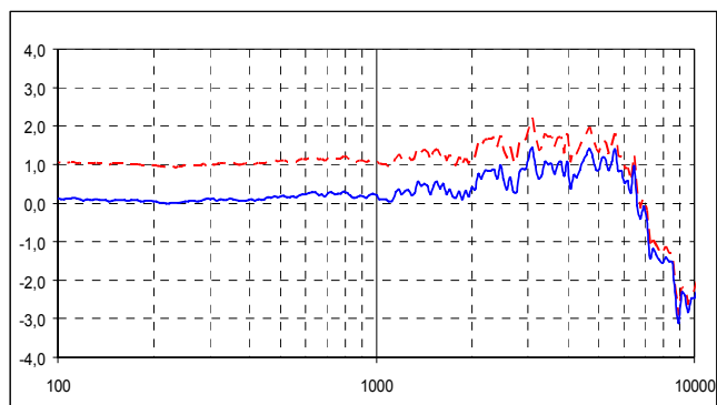
Fig. 16: corresponding frequency response
