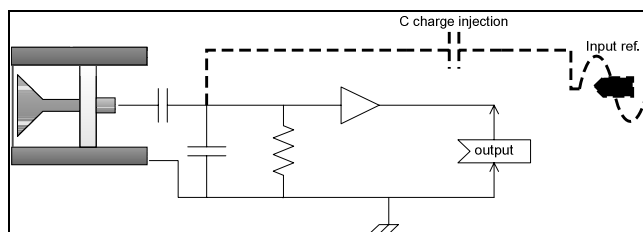
Fig 3: charge injection principle
