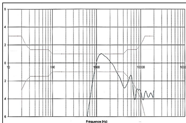
Fig. 2: corresponding frequency response
