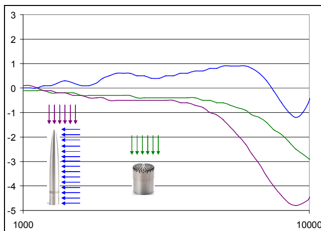
Fig. 9: electronic corrections implemented in DUO
