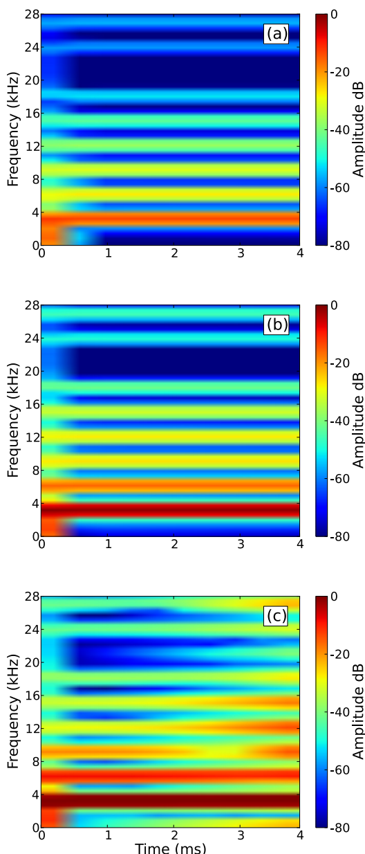
Figure 5: Spectrograms of simulated tone F\#7 ( f=2960 Hz) calculated for constant value of the capo bar curvature R = 1 mm, and varying the hammer striking velocity V . (a) V = 1 m/s, (b) V = 2 m/s, (c) V = 3 m/s.
