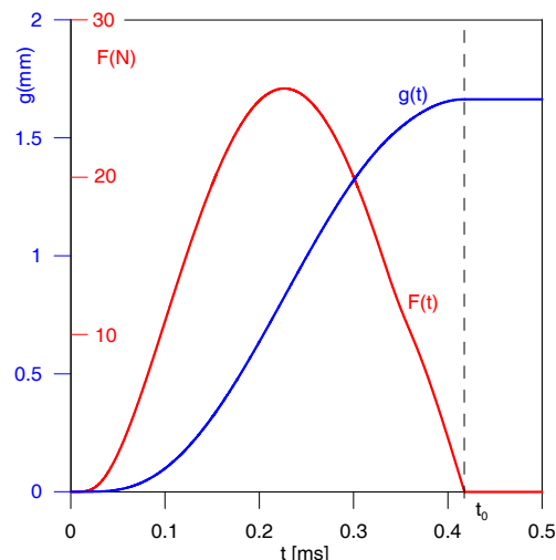
Figure 1: Force history and g function computed for tone F\sharp 7 ( f = 2960 Hz). The dashed line defines duration of contact t_0 .
