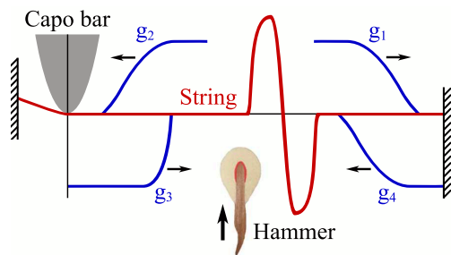
Figure 2: Scheme of capo bar-string interaction. Functions g are the traveling waves.
