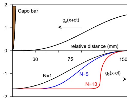
Figure 3: Distortion of the form of reflecting wave g_3 after several number of rereflections N = 1; 5; 13 , shown in different colors.
