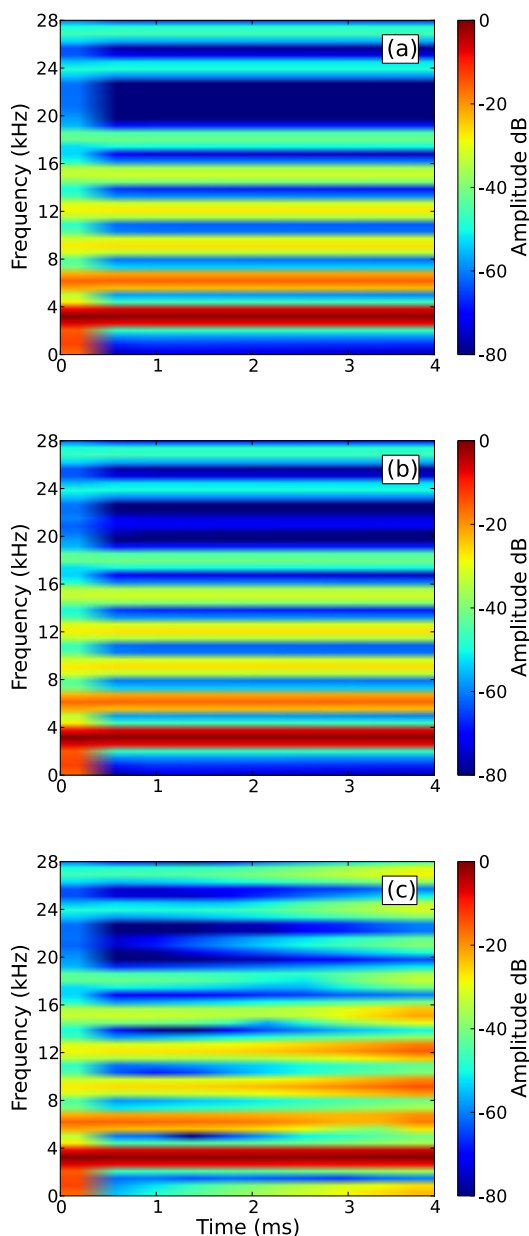
Figure 4: Spectrograms of simulated tone F\sharp 7 ( f = 2960 Hz) calculated for constant value of hammer striking velocity V = 2 m/s, and varying radius of the capo bar curvature R . (a) R = 0 , (b) R = 1 mm, (c) R = 2 mm.
