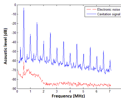
Figure 2: Example of instantaneous acoustic spectrum induced by a fixed intensity of 2.7 W/cm 2 and the reference noise which is subtracted to provide the inertial cavitation level.
