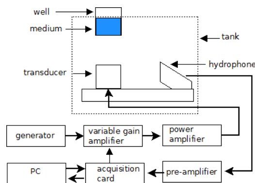
Figure 1: Experimental setup
