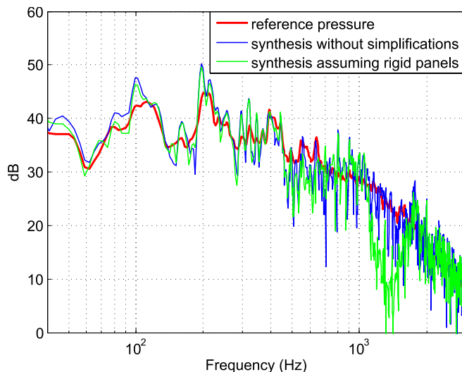
Figure 5: Example of measured reference pressure (red) and synthesized reference pressure assuming rigid panels (green) and without making any assumption (blue) in a car interior.
