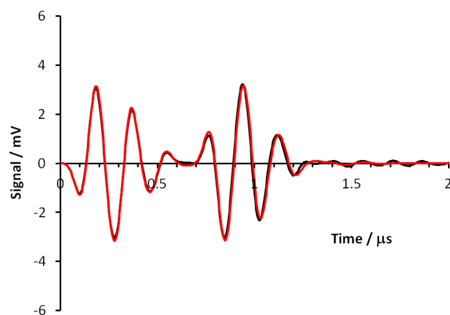
Figure 3: Time-domain results for discrete scatterer model (black) and effective medium model (red) for 5 \text{ }\mu\text{m} radius cavities at 10\% v/v with a 5 \text{ MHz} centre-frequency signal (scaled by concentration).
