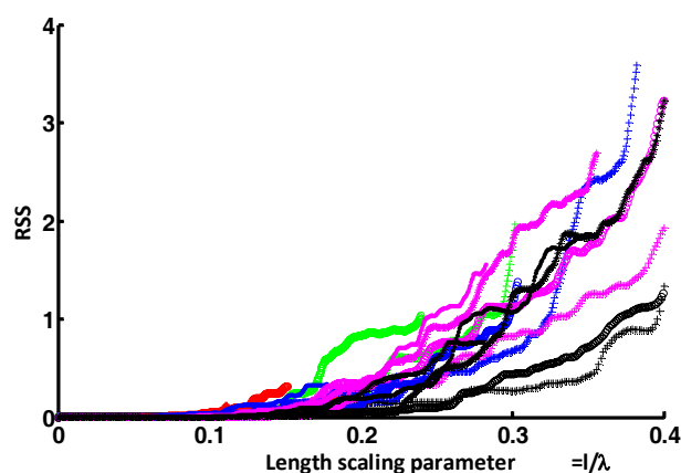
Figure 6: RSS plotted against length scale parameter l/\lambda for all sets of radii and concentration for the discrete scatterer model single realizations. Radii [5,7.9,10,15.9,20 \mu\text{m} ] are denoted by colours in sequence [red, green, blue, magenta, black] and symbols [+ , \circ , * , . , \times ] denote concentrations [1,2,5,10,20%].
