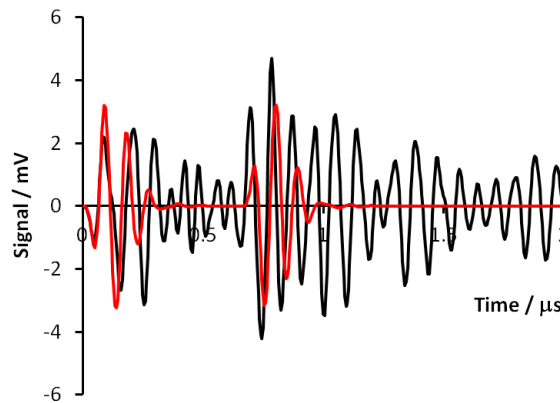
Figure 2: Time-domain results for discrete scatterer model (black) and effective medium model (red) for 10 \text{ }\mu\text{m} radius cavities at 2\% v/v with a 10 \text{ MHz} centre-frequency signal (scaled by concentration).
