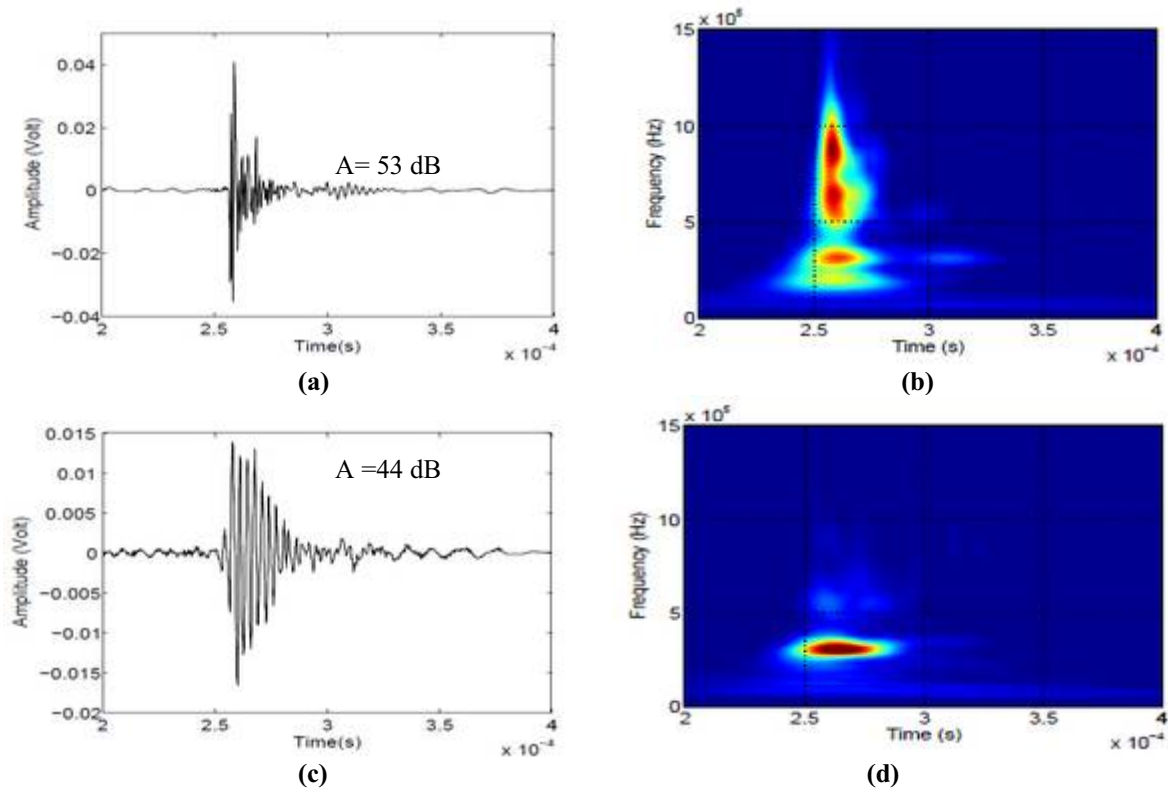
Figure 6: Time-amplitude representation (a, c) and Time-frequency content (b, d) of typical AE signal recorded from 90° specimen test. The first signal is related to interfacial damage, the second is relate to matrix cracking damage.
