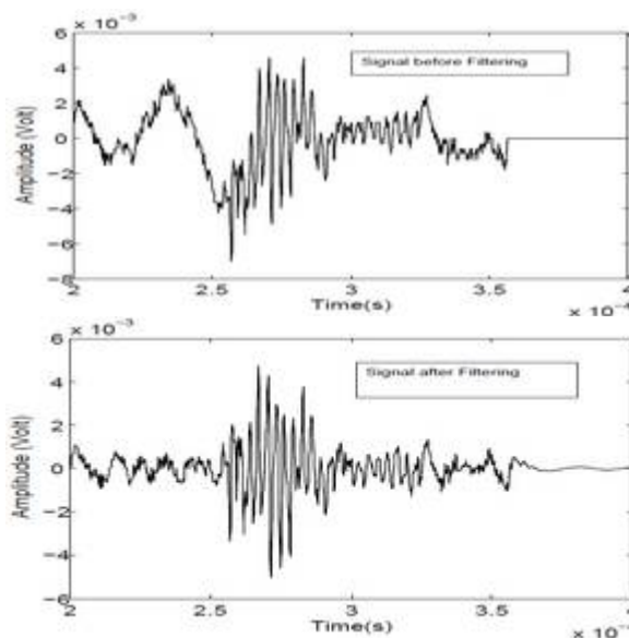
Figure 3: Effect of the wavelet transform filtering.
