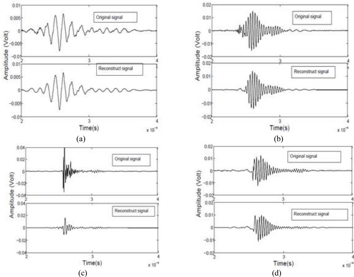
Figure7 : Reconstruction of AE signals: Projection on the matrix cracking dictionary, (a, b) model signals acquired from test on resin, (c, d) model signals acquired from test on 90° UD-GFRP composite.
