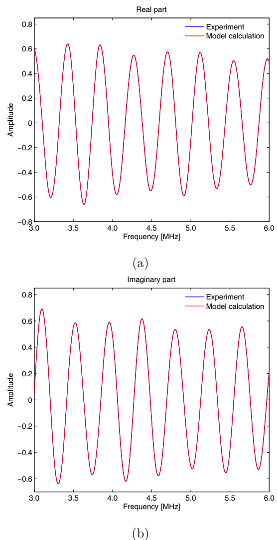
Figure 4: Complex transmission of a 8 mm Plexiglas plate calculated and measured in the 3-6 MHz frequency range: (a) real and (b) imaginary parts.
