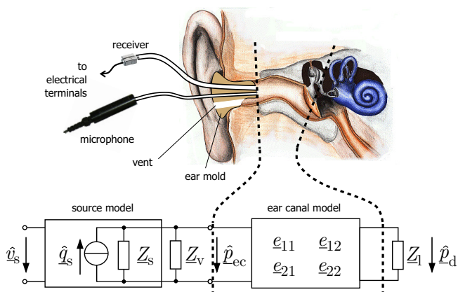
Figure 1: Model framework for the prediction of the sound pressure \hat{p}_d at the drum, in ear canals with vented ear molds.
