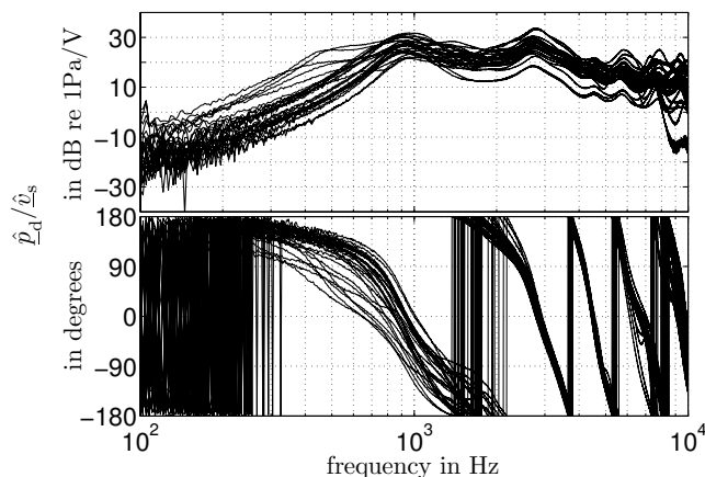
Figure 3: Sound pressure relative to the source voltage measured at the ear drum for the 28 ears.
