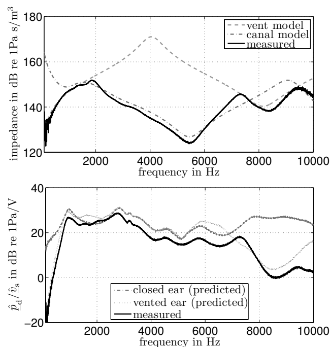
Figure 5: Example for the influence of the vent on the impedance and the sound pressure. On top, impedances of a vent model, of an occluded ear canal model, and the corresponding measured impedance of a vented ear. Below, transfer functions of sound pressure relative to the source voltage for a prediction of the occluded ear, a prediction of the vented ear and the measured transfer function.
