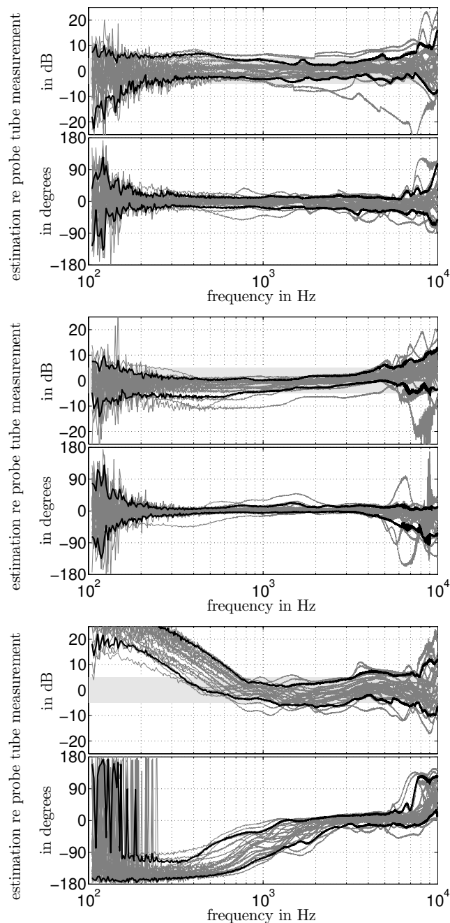
Figure 4: Level and phase differences of the predicted relative to the measured sound pressure at the ear drum. Top: method using independent models, middle: method using joint models, bottom: ear simulator model. The gray lines are the individual data, the black lines give the 10th and the 90th percentile.
