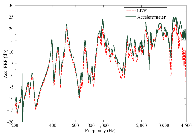
Figure 7: Acceleration FRFs of the violin suspended free-free excited with an impulse hammer and measured with (red) LDV, and (green) accelerometer. The result of the LDV has been differentiated to be comparable with the one of the accelerometer
