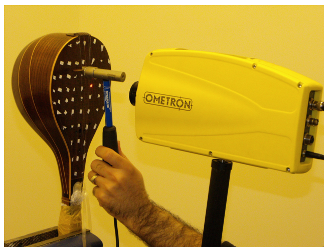
Figure 2: The experimental setup for modal analysis of the clamped setar using an impulse hammer and LDV.
