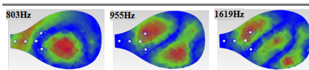
Figure 6: Extra modes appeared in the results when measuring with an accelerometer. The setar is clamped in a stiff vice and is excited by an impulse hammer
