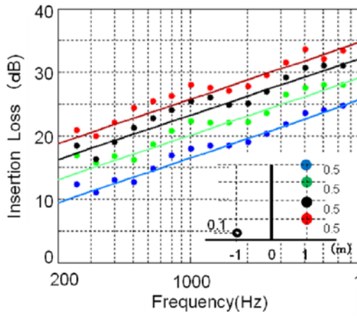
Fig. 4.1 Comparison of the insertion loss of the flat top edge between measurement (circle) and calculation (solid line).
