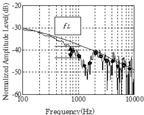
Fig. 2 Measurement example of the cut-off frequency f_L
