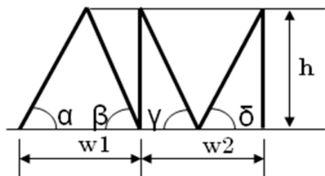
Fig. 1 Geometric parameters of M shaped noise barrier.
