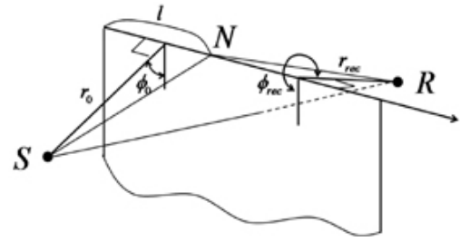
Fig. 6 Geometrical parameters of Eq. (1) and (2).
