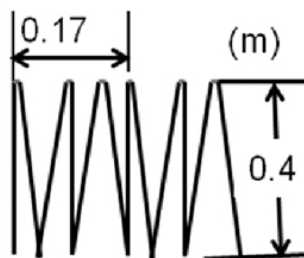
Fig. 5 M shaped wedge test specimen for anechoic measurement.
