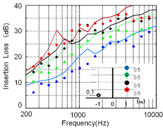
Fig. 4.2 Comparison of the insertion loss of M shaped edge between the measurement (circle) and calculation (solid line).
