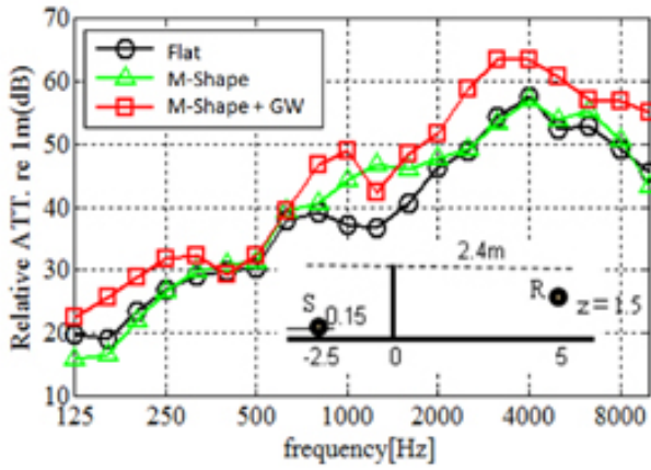
Fig. 7 Measurement example of the relative attenuation (re. 1 m in free field) of flat edge barrier and M shaped barrier with / without glass wool board behind. The shape parameter of the latter is h = 340 mm, w_1 = w_2 = 360 mm, and \alpha = \beta = \gamma = \delta = 62^\circ .
