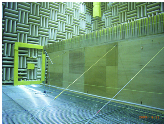
Fig. 3 Anechoic measurement.
