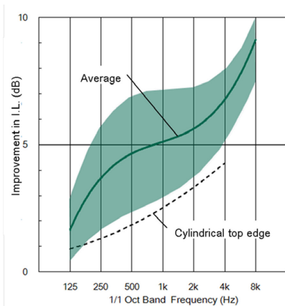
Fig. 8 Measured variation range of the improvement in the insertion loss of M shaped barrier with grass wool behind compared to flat top barrier with same height. The dotted line means expected value of the cylindrical top edge barrier.
