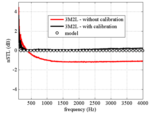
Figure 4: nSTL of the 80mm air layer.
