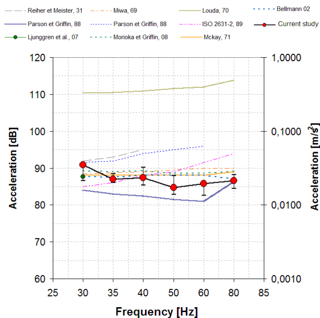
Figure 3: The median and the inter-quartile range (25-75th percentiles) of absolute threshold of whole-body vertical vibration, some data are based on [2] and [3].
