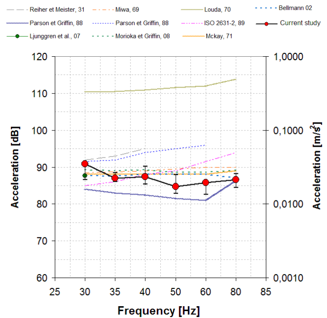
Figure 3: The median and the inter-quartile range (25-75th percentiles) of absolute threshold of whole-body vertical vibration, some data are based on [2] and [3].
