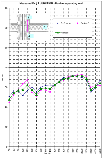
Figure 8: Measured T junction Floor-Façade. Paths 3-4.
