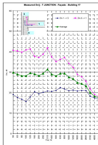
Figure 5: Measured T junction Floor-Façade. Paths 1-3.
