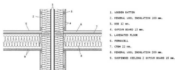
Figure 1: Elements composing the Floor and Double Separating Wall Junction
