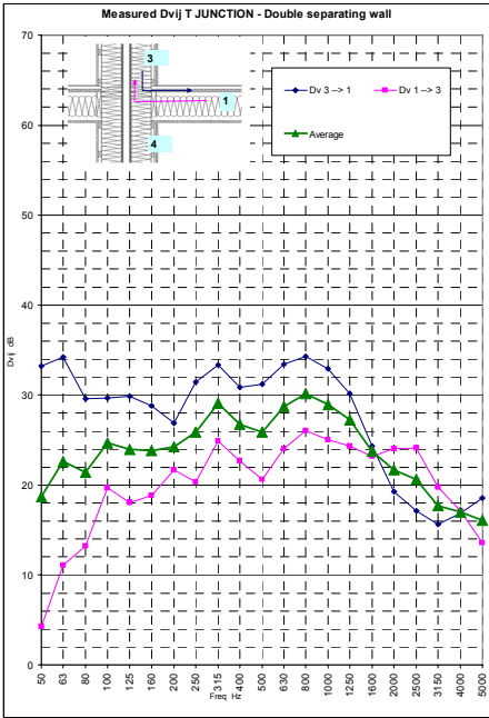
Figure 9: Measured T junction Floor-Façade. Paths 1-3.
