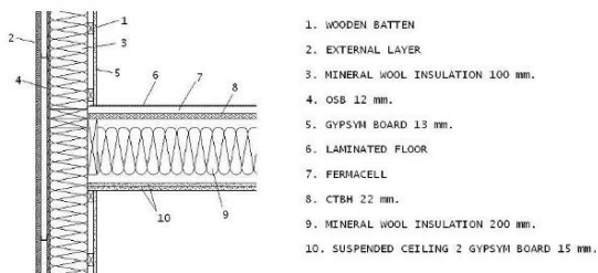
Figure 3: Elements composing the Floor and Façade Junction
