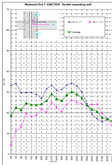
Figure 9: Measured T junction Floor-Façade Double separating wall. Paths 1-3.
