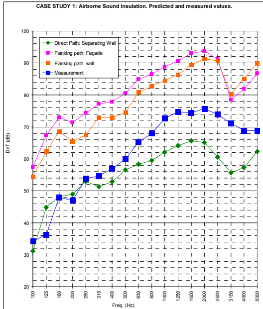
Figure 11: Case Study 1. Airborne sound insulation Comparison of predicted and measured values
