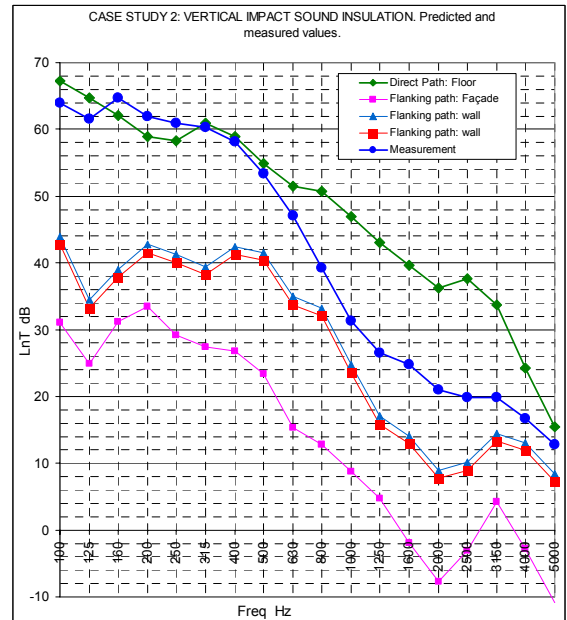
Figure 12: Case Study 2. Impact sound insulation Comparison of predicted and measured values
