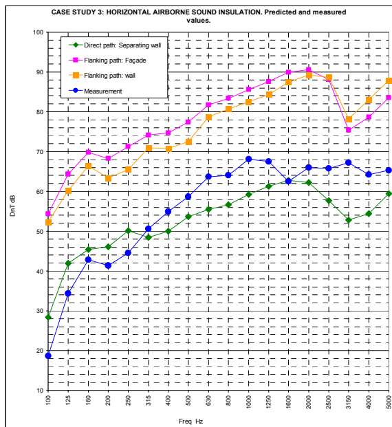
Figure 13: Case Study 3. Airborne sound insulation Comparison of predicted and measured values
