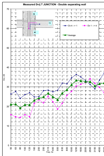
Figure 10: Measured T junction Floor-Façade Double separating wall. Paths 1-4.
