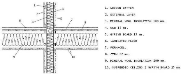
Figure 2: Elements composing the Floor and Single Wall Junction
