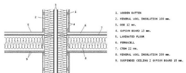
Figure 1: Elements composing the Floor and Double Separating Wall Junction
