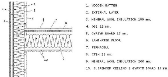
Figure 3: Elements composing the Floor and Façade Junction
