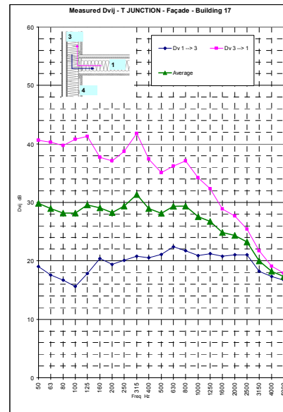
Figure 5: Measured T junction Floor-Façade. Paths 1-3.
