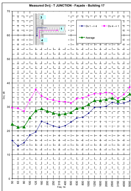
Figure 7: Measured T junction Floor-Façade. Paths 1-4.
