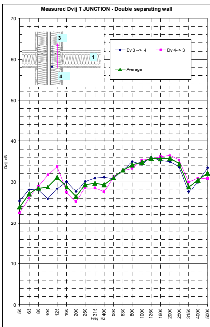
Figure 8: Measured T junction Floor-Façade Double separating wall. Paths 3-4.
