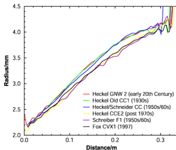
Figure 1: Bore profiles of six bassoon crooks.
