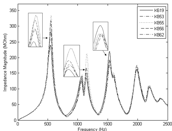
Figure 2: Input impedance magnitude curves for five Howarth student model oboes with F6 fingering applied.
