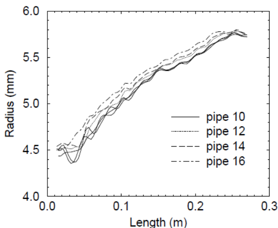
Figure 6: Bore profiles of four trumpet leadpipes in the mandrel I family. Three replicas of pipe 10 are shown.
