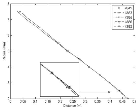
Figure 3: Bore profiles of the bottom and top joints of five Howarth student model oboes.
