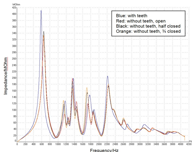
Figure 4: Input impedance magnitude curves for Howarth oboe with standard C7 fingering applied together with different degrees of venting.
