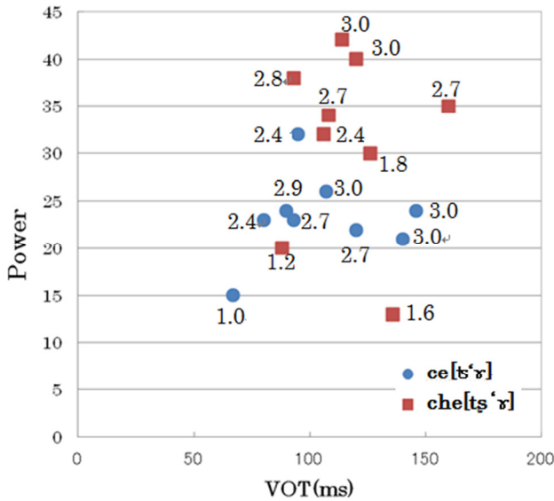
Figure 6: Data distributions on the surface of VOT and power with the score of students' pronunciation of aspirated retroflex che[t\text{'}\text{ɻ}] and aspirated dental ce[t\text{'}\text{ɻ}] .
