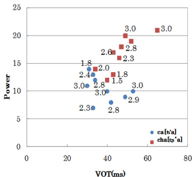
Figure 4: Data distributions on the surface of VOT and power with the score of students' pronunciation of aspirated retroflex cha[t\zeta'a] and aspirated dental ca[t's'a] .
