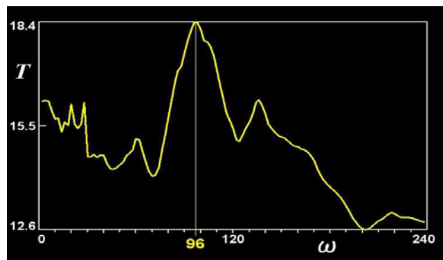
Figure 12: Objective function and optimum value \omega .
