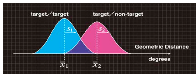
Figure 11: Distributions of geometric distances.
