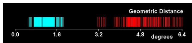
Figure 13: Distributions with optimum value \omega=96 .
