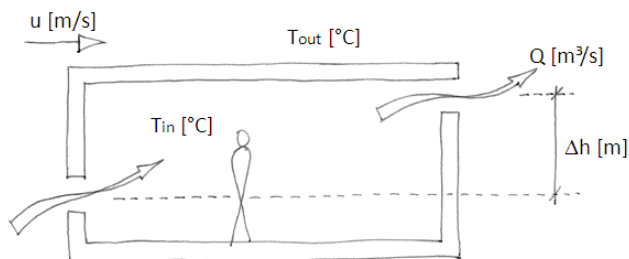
Figure 3: Naturally ventilated room with ventilation openings on two facades.
