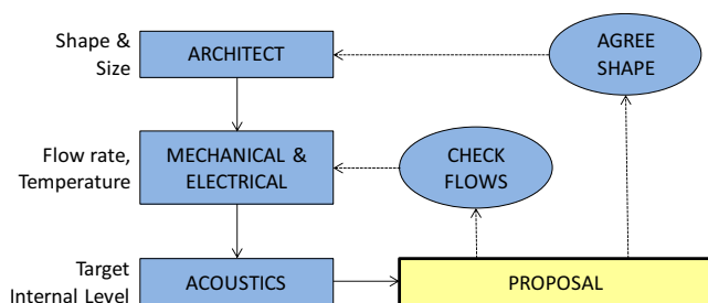
Figure 2: Design process for attenuated natural ventilation.
