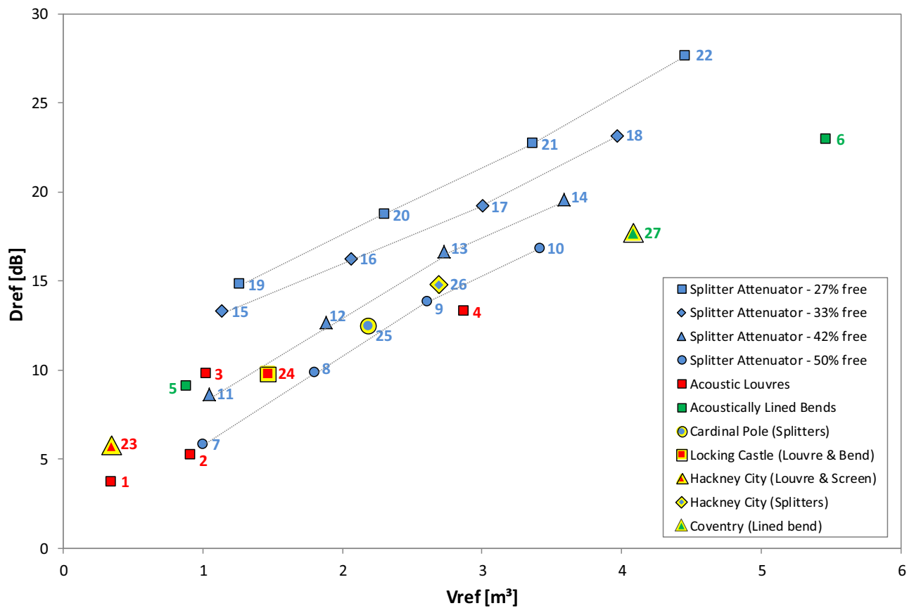
Figure 4: Plot of D_{ref} vs V_{ref} for 27 acoustically attenuated ventilators.
