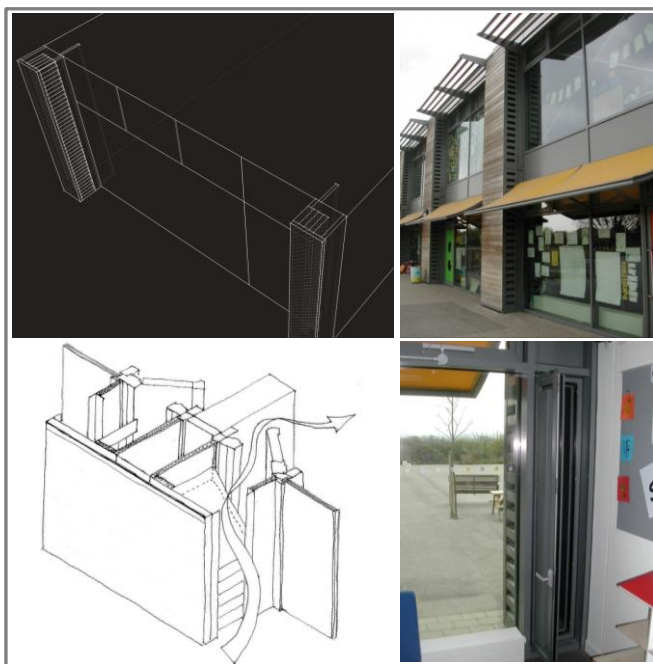
Figure 5: Acoustic louvres at Locking Castle School
