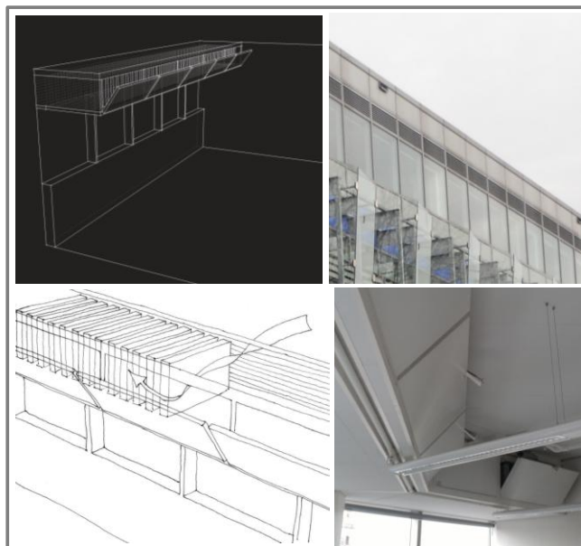
Figure 7: Splitter attenuator at the City Academy, Hackney
