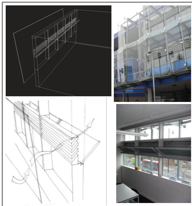
Figure 6: Acoustic louvres at the City Academy, Hackney
