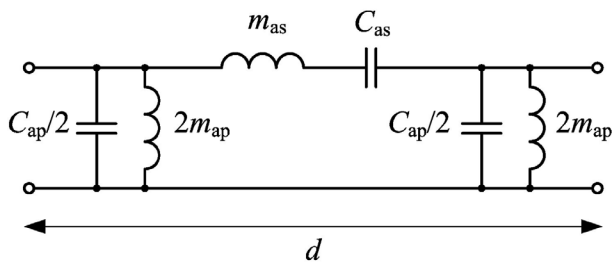
Figure 2: Lumped element model of the \Pi -type unit-cell of the transmission-line acoustic metamaterial
