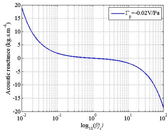
Figure 5: Example of achievable active reactance.
