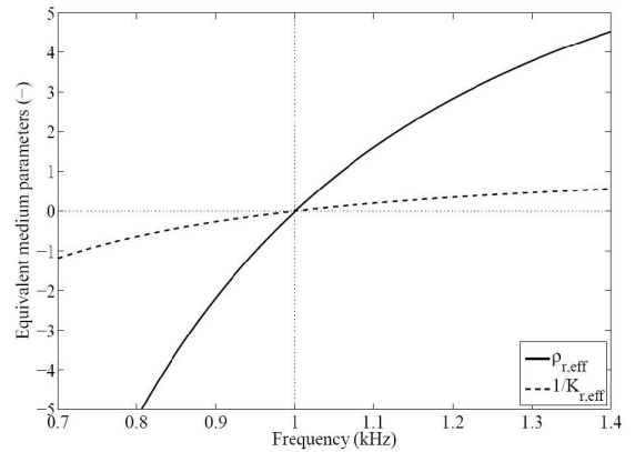
Figure 3: Equivalent mass density and bulk modulus (relative values) for the considered CRLH TL around the transition frequency
