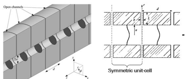
Figure 1: Acoustic transmission-line metamaterial concept, composed on periodic inclusions of elastic membranes (black disks) and radial open channels (“stubs”). Left: isometric view of the structure; right: cut-view of 2 unit-cells of the structure.
