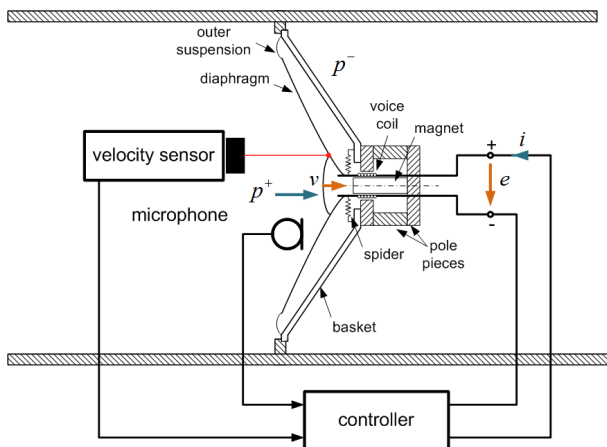
Figure 4: Sketch of an electrodynamic loudspeaker with direct impedance control.
