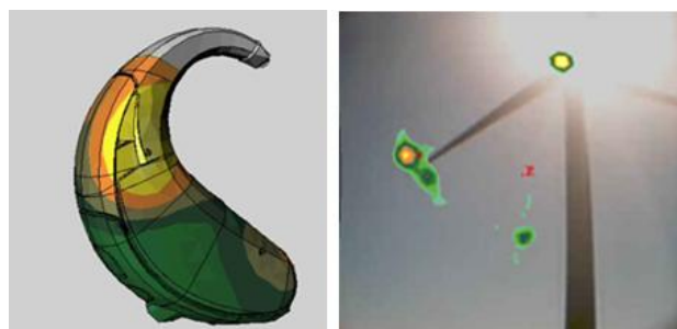
Fig.11. Left: Conformal sound intensity map on a hearing aid at 2400Hz. Right: refined beamforming sound intensity map on wind turbine at 4000Hz
