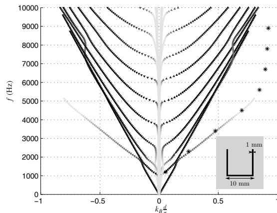
Figure 2: Band diagram for U-shape inclusions. The gray scale indicates the magnitude of the imaginary part of k_B . The darkest are the line the smallest is the imaginary part.
