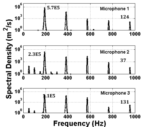
Figure 4: The data of figure 2 plotted in frequency domain
