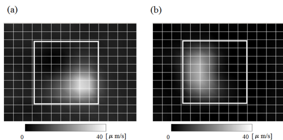
Fig. 9: Examples of the vibration velocities images which the buried object is buried diagonally. A styrofoam board ( 300 \times 300 \times 25 \text{ mm}^3 ) is used. Average buried depth is 15 mm, but the upper side depth is 9 - 10 mm and lower side depth is 20 - 21 mm. (a) Imaging frequency is 1553.5 Hz, (b) Imaging frequency is 1422.5 Hz.
