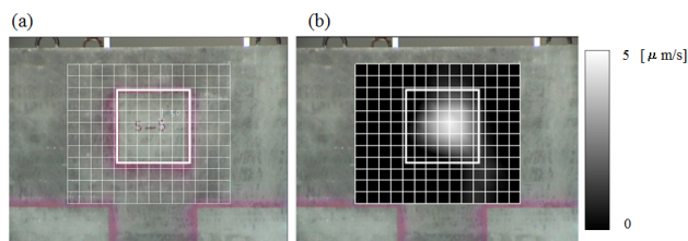
Fig. 6: Experimental result. A styrofoam board ( 300 \times 300 \times 25 \text{ mm}^3 ) is buried in 50 mm depth of the concrete test piece. (a) Scan area and position of the buried object by CCD, (b) The vibration velocity distribution imaging result by SLDV. Chirp (1800-2400 Hz) is used, imaging frequency is 2004 Hz.
