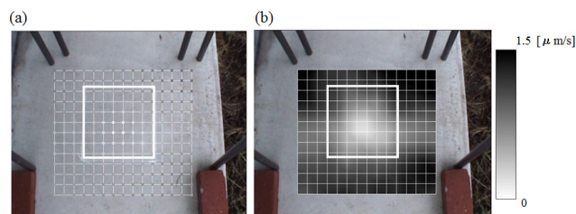
Fig. 4: Experimental result. A styrofoam board ( 300 \times 300 \times 150 \text{ mm}^3 ) as a substitute for a cavity at the depth of 50 mm. The sound pressure is about 110 dB near the surface of the concrete test piece. The white flame shows the size and the position of a styrofoam. (a) Scan area and position of buried object by CCD camera, (b) Imaging result by SLDV. Imaging frequency : 2198 Hz. Output wave : Linear chirp (2100 – 2500 Hz).
