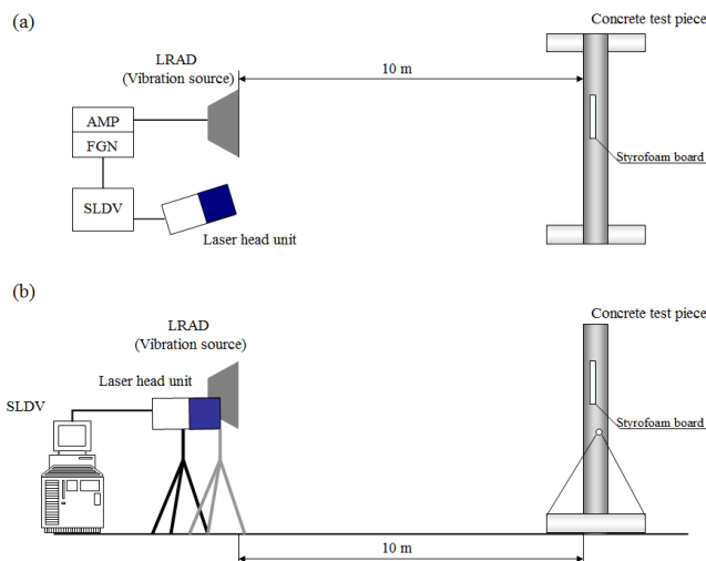
Fig. 5: Experimental setup for long distance emission using a concrete test piece. The distance between the LRAD and the concrete test piece is 10 m. Number of scan point is 195 ( 13 \times 15 ). Dimension of the scan area is changed by the size of the buried object. (a) upper view, (b) side view.
