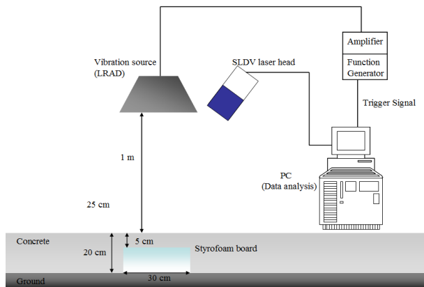
Fig. 2: Experimental setup for inspection possibility test using a concrete tests piece. A styrofoam ( 300 \times 300 \times 150 \text{ mm}^3 ) as a substitute for a cavity are buried in the concrete. The distance between concrete surface and buried object is 50mm
