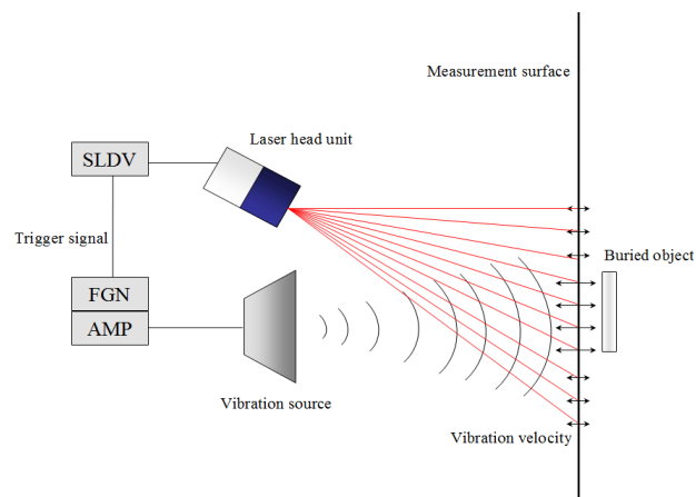
Fig.1: Fundamental concept of NCAI.
