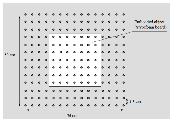
Fig. 3: Dimensions of scan area ( 500 \times 560 \text{ mm}^2 ). The number of the scan points is 195 ( 13 \times 15 ).
