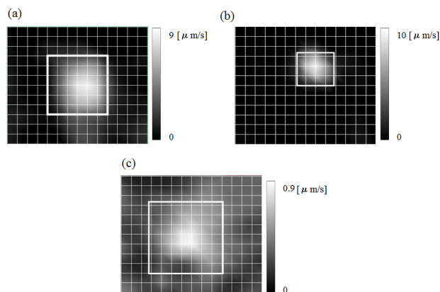
Fig. 7: Experimental results of the vibration velocity distribution image. (a) A styrofoam board ( 200 \times 200 \times 25 \text{ mm}^3 ) is buried in 45 mm depth, imaging frequency is 2800 Hz, (b) A styrofoam board ( 100 \times 100 \times 25 \text{ mm}^3 ) is buried in 25 mm depth, imaging frequency is 4000 Hz, (c) A styrofoam board ( 500 \times 500 \times 25 \text{ mm}^3 ) is buried in 75 mm depth, imaging frequency is 1187.5 Hz.
