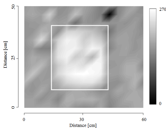
Fig. 10: An applying example of the optimum frequency range method (OFR method). In this case, frequency range from 1300 to 1600 Hz are integrated .
