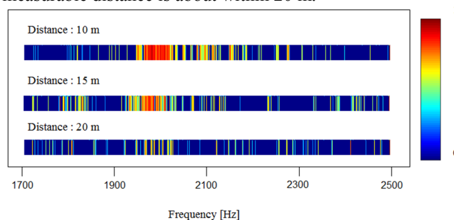
Fig. 8: Brightness image of the frequency response of the vibration velocity. The distance between a concrete test piece and a LRAD is 10, 15 and 20 m.
