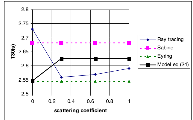
Figure 1: Reverberation time T30 computed by four models in a cubic room with L=10m and \alpha=0.1 . The scattering coefficient is the same for all surfaces and its value is one of the following {0, 0.3, 0.65, 1}.
