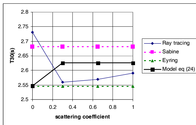
Figure 1: Reverberation time T30 computed by four models in a cubic room with L=10m and \alpha=0.1 . The scattering coefficient is the same for all surfaces and its value is one of the following \{0, 0.3, 0.65, 1\} .
