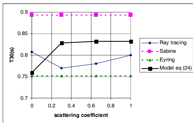
Figure 2: Same as figure 1 with \alpha=0.3 .
