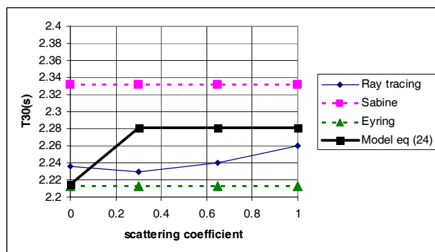
Figure 3: Reverberation time T30 computed by four models in an irregular room ( V=733\text{m}^3 , S=506\text{m}^2 ) and \alpha=0.1 . The scattering coefficient is the same for all surfaces.
