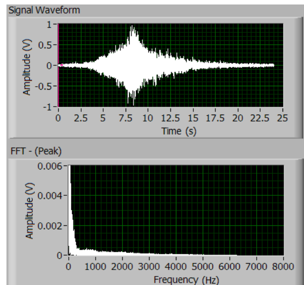
Figure 6: Typical Noise and Spectrum Signal of a 747 taking off.
