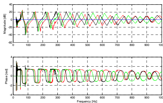
Figure 6: Measured impedance (magnitude and phase as a function of frequency) of the Tintignac carnyx copy (red), and with a calculated extension of 10 cm (green) and of 20 cm (black).
