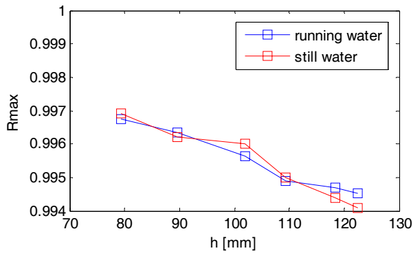
Figure 5: Mean of the six maximums of the CCF as a function of water level.
