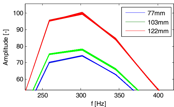
Figure 6: Frequency spectrum maximal points for three flow water levels.
