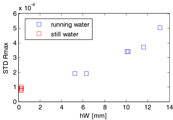
Figure 6: Standard deviation of the six maximums of the CCF as a function of surface water waves amplitude.
