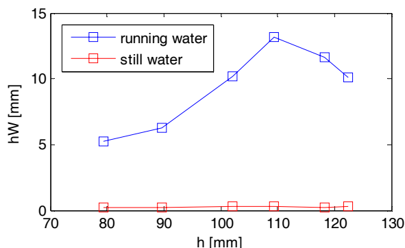
Figure 3: Time-averaged surface water waves amplitude as a function of time-averaged water level height.
