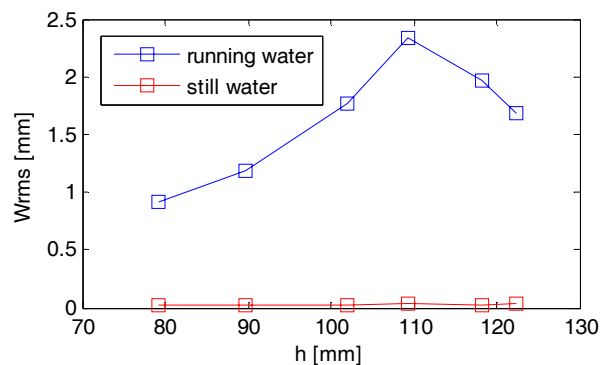
Figure 4: Root mean square of the water surface roughness as a function of time-averaged water level height.
