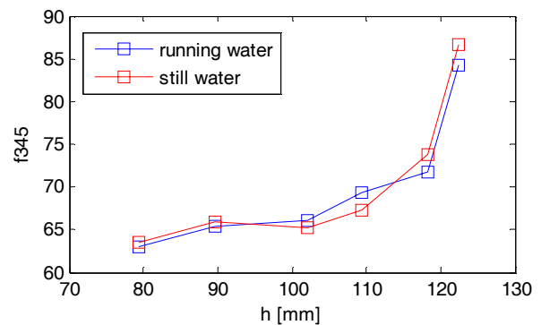
Figure 7: Mean of frequency spectrum values at 345Hz as a function of time-averaged water level height.
