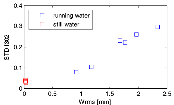
Figure 8: Standard deviation of the probability density function as a function of water surface waves RMS.
