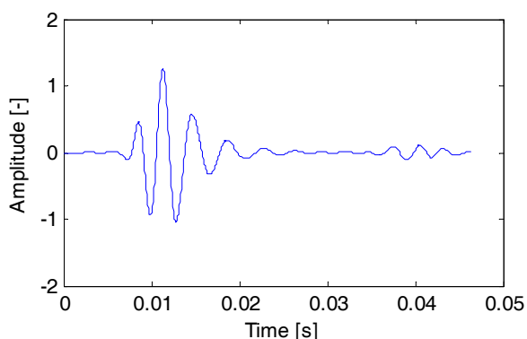
Figure 2: Filtered acoustic pulse for 86mm water flow.
