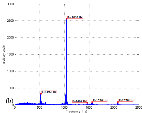
Figure 3: Spectrum of the pressure signal (a) Re=12350, (b) Re=18200.
