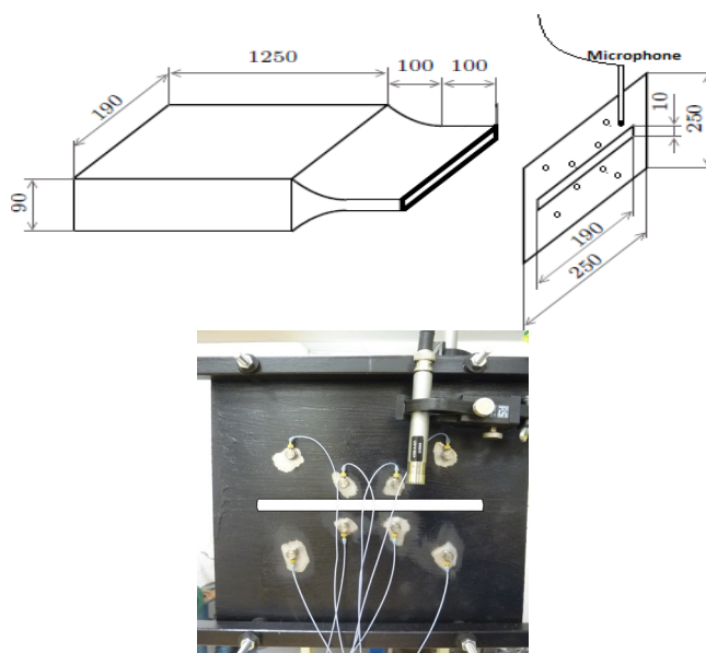
Figure 1: Experimental apparatus
