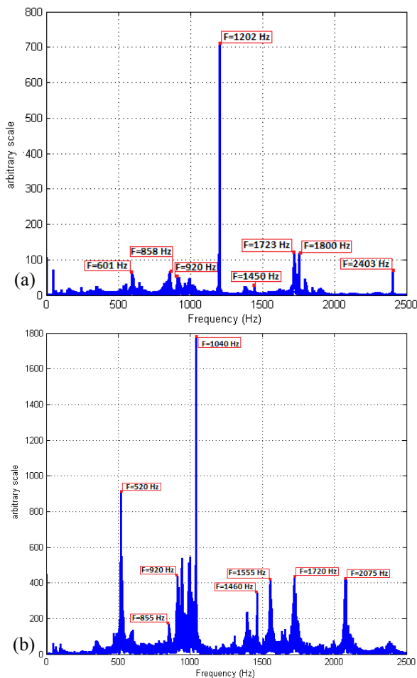
Figure 2: Spectrum of the plate vibration (a) Re=12350, (b) Re=18200.
