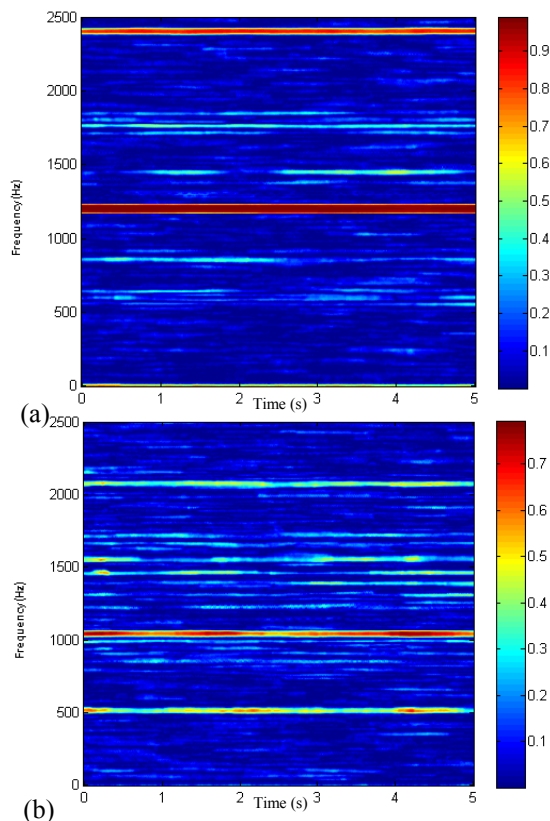
Figure 4: Coherence 'frequency-time' between the pressure and the vibration signals (a) Re=12350, (b) Re=18200.
