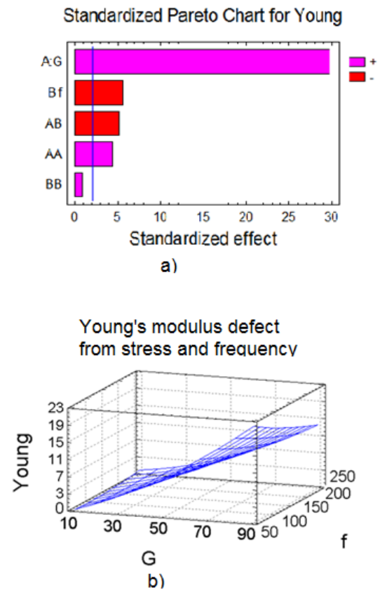
Figure 2: a) The effect of coefficients on the response function in the first model for defect Young's modulus dependences from stress and frequency; b) Response function surface for the first model.
