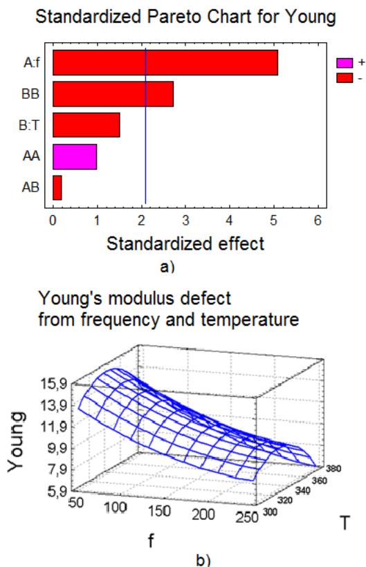
Figure 4: a) The effect of coefficients on the response function in the third model for defect Young's modulus dependences from frequency and temperature; b) Response function surface for the second model.
