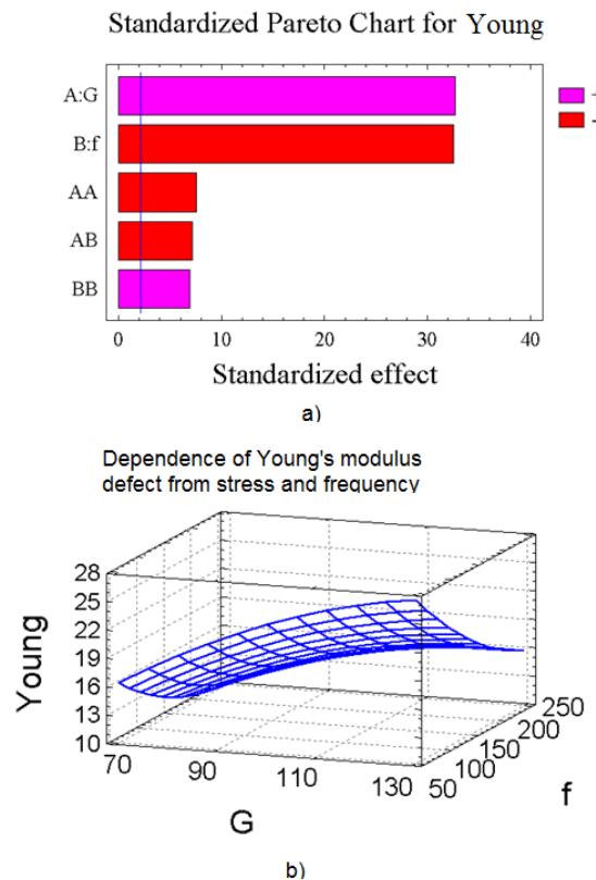
Figure 3: a) The effect of coefficients on the response function in the second model for defect Young's modulus dependences from stress and frequency; b) Response function surface for the second model.
