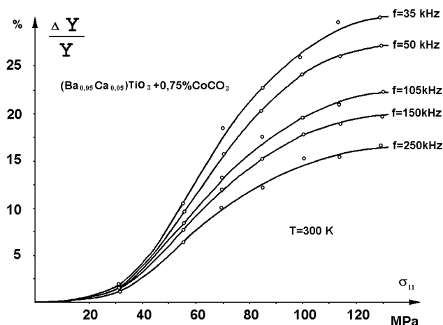
Figure 1: The Young's modulus defect on stress.
