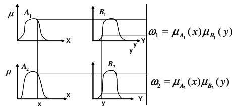
Figure 6: First-order Sugeno fuzzy model.
