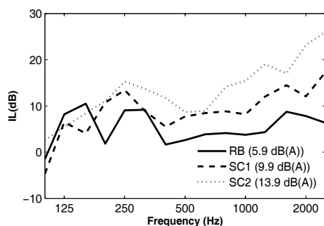
Figure 6: Insertion loss of rigid and sonic crystal noise barriers as a function of frequency: tramway noise. RB (solid line), SC1 (dashed line) and SC2 (dotted line).
