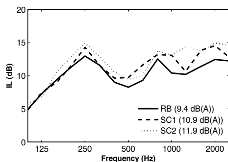
Figure 5: Insertion loss of rigid and sonic crystal noise barriers as a function of frequency: road traffic noise. RB (solid line), SC1 (dashed line) and SC2 (dotted line).
