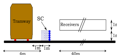
Figure 4: Geometrical configuration for tramway noise.
