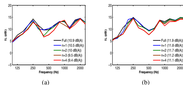
Figure 8: Insertion loss of sonic crystals SC1 (a) and SC2 (b) for the different orders of scatterers number reduction ( IL_{RB}=9.4 dB(A)): road traffic noise.
