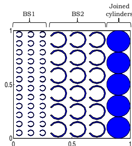
Figure 2: Scatterers arrangement in the low height sonic crystal noise barrier.
