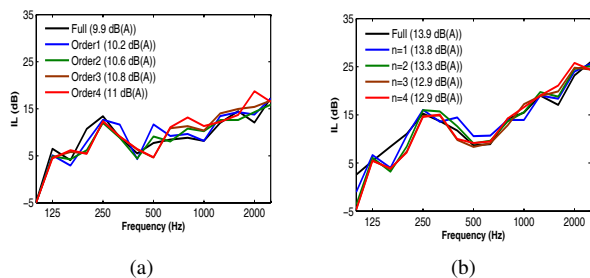
Figure 9: Insertion loss of sonic crystals SC1 (a) and SC2 (b) for the different orders of scatterers number reduction ( IL_{RB}=5.9 dB(A)): tramway noise.
