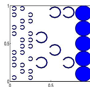
Figure 7: Sonic crystal barrier obtained for the fourth order of scatterers number reduction.
