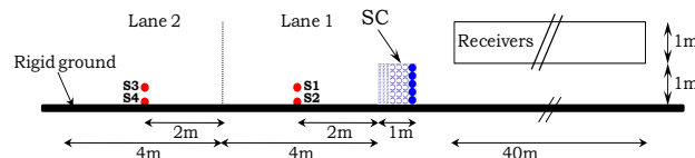
Figure 3: Geometrical configuration for road traffic noise.
