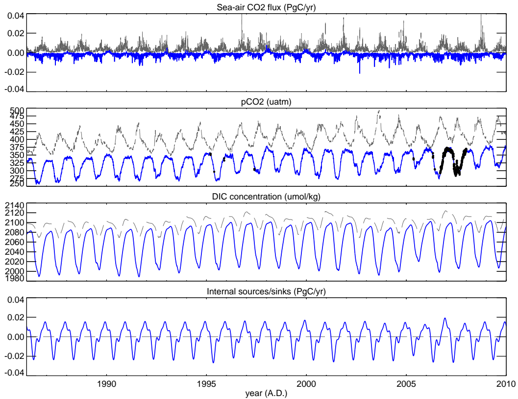
Fig. 3. Example time series (full daily resolution) at the model pixel around Station M ( 66^\circ\text{N} , 2^\circ\text{E} ) of the main quantities of the diagnostic model (Fig. 1): sea–air \text{CO}_2 fluxes ( f_{\text{ma}}^{\text{CO}_2} ), surface-ocean \text{CO}_2 partial pressure ( p_{\text{m}}^{\text{CO}_2} ), mixed-layer DIC concentration ( C_{\text{m}}^{\text{DIC}} ), as well as ocean-internal carbon addition to (removal from) the mixed layer ( f_{\text{int}}^{\text{DIC}} ). Estimates have been obtained by fitting the diagnostic scheme to SOCAT surface-ocean \text{CO}_2 partial pressure data (SFC, blue). The SOCAT data points that happen to fall in the example pixel are shown as black dots in the p_{\text{m}}^{\text{CO}_2} panel. The Bayesian prior ( f_{\text{int}}^{\text{DIC}} = 0 and corresponding C_{\text{m}}^{\text{DIC}} , p_{\text{m}}^{\text{CO}_2} , and f_{\text{ma}}^{\text{CO}_2} , Appendix A2.2, Sect. 3.2) is also given (thin dashed grey lines).
