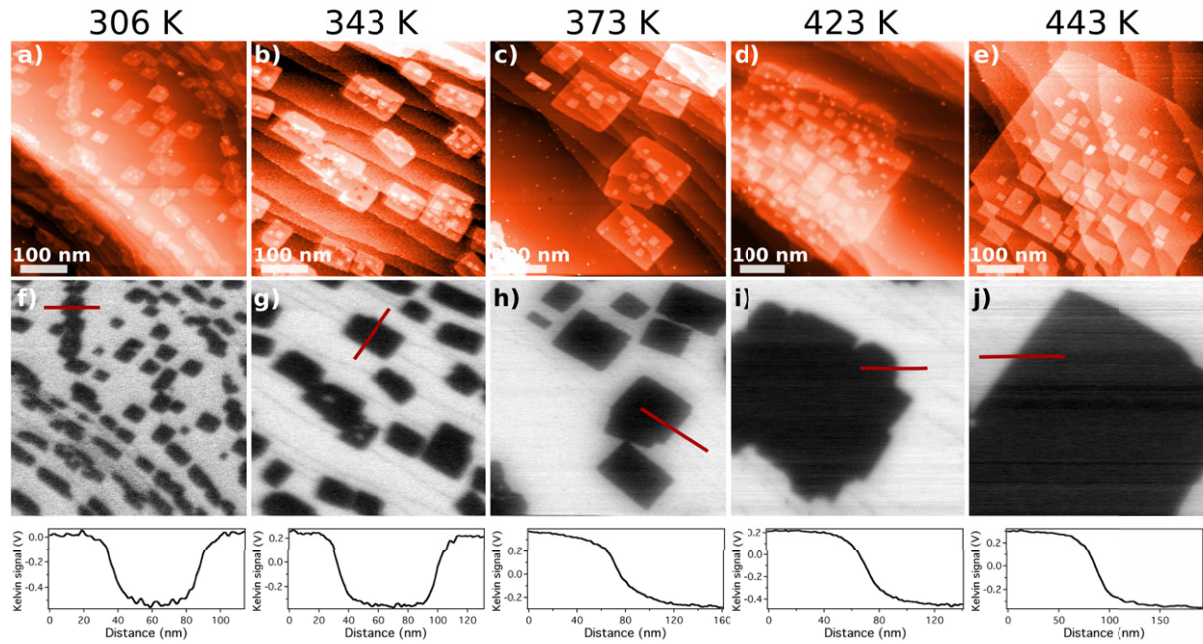
Figure 1. nc-AFM (top) and KPFM (bottom) images of 0.75 MLE thin NaCl films grown on Ag(001) held at various temperatures as indicated above each column. Each film was separately grown after cleaning the Ag(001) substrate by sputtering and annealing. The line profiles of the Kelvin images were taken over the edges of the islands and represent the WF change between Ag(001) and NaCl/Ag(001). Imaging parameters: 500 \times 500 \text{ nm}^2 , speed = 0.5 Hz, A = 22 \text{ nm} , f_{ac} = 474 \text{ Hz} , U_{ac} = 150 \text{ mV} (d, i: 250 mV and e, j: 100 mV). \Delta f (Hz) = -19 (a), (c), (f), (h); -8 (b), (g); -49 (d), (i); and -17 (e), (j).
