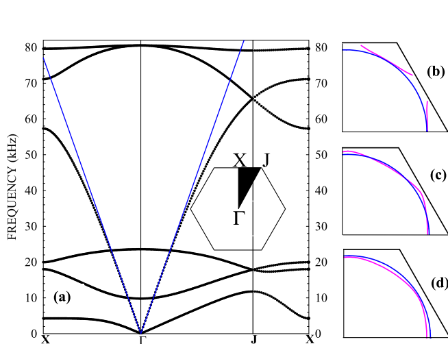
FIG. 2. (a) Dispersion curves in the first Brillouin zone, along the \Gamma/JX path. The slope of the blue lines is the wave velocity in water. EFCs of the MWS represented in the right upper quadrant of the hexagonal Brillouin zone (the 3 other quadrants can be redrawn by symmetry). (b) 70.8 kHz, (c) 71.2 kHz, and (d) 71.6 kHz (pink). The blue circle corresponds to the EFC in water and the black lines to the Brillouin zone.
