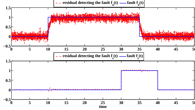
Figure 12: Fault estimation
