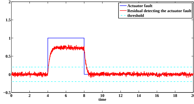
Figure 4: Residual generator 2 : Actuator fault detection
