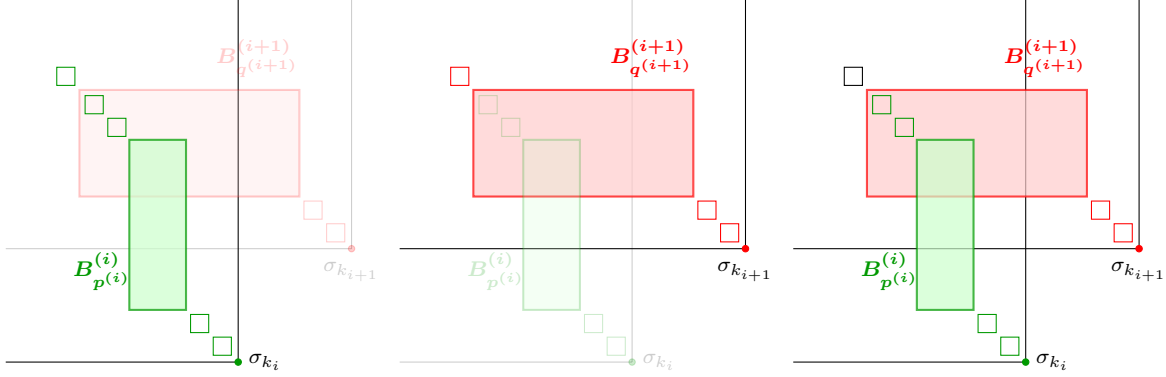
Figure 7: Block decomposition of \sigma^{(i)} and of \sigma^{(i+1)} when p^{(i)} > q^{(i+1)}
