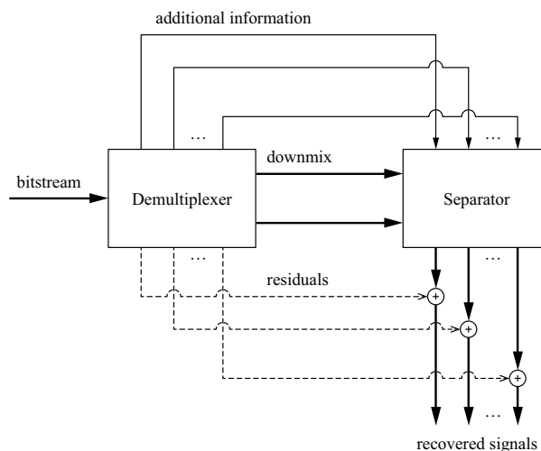
Fig. 2: General architecture of an ISS decoder.
