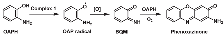
Scheme 2 Probable mechanism for the formation of the phenoxazinone chromophore.
