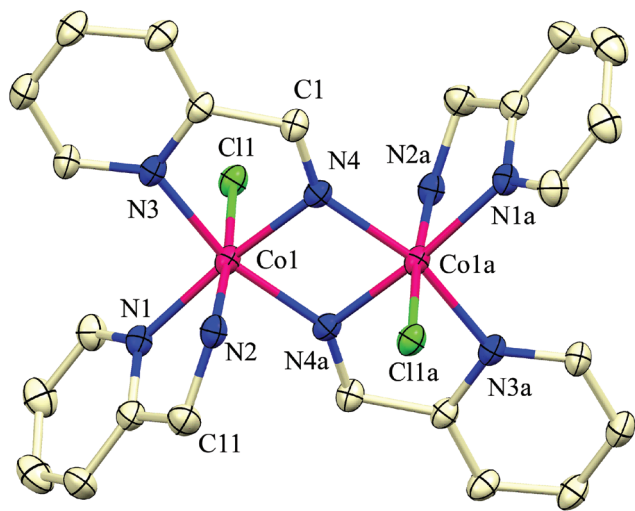
Fig. 1 ORTEP diagram of complex cation 1 showing the atom numbering scheme. Ellipsoids are drawn at the 50% probability level. H atoms are omitted for clarity. Symmetry code: a = 1 - x, -y, 1 - z .
