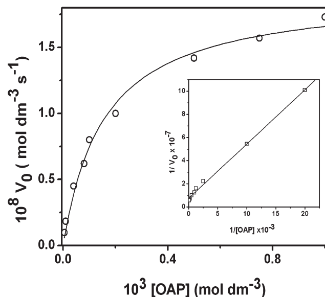
Fig. 5 Plot of the initial rates at the OAPH concentrations for the oxidation reaction catalyzed by the complex at a fixed concentration in dioxygen-saturated methanol at 25 °C. The inset shows the reciprocal Lineweaver–Burk plot.
