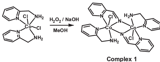
Scheme 1 Schematic representation of the synthesis of the dinuclear complex.
