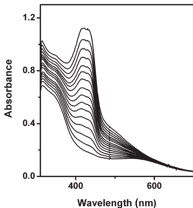
Fig. 4 Time resolved UV-vis spectral changes for the oxidation of 2-aminophenol ( 5 \times 10^{-3} mol \text{dm}^{-3} ) catalyzed by the complex ( 5 \times 10^{-5} mol \text{dm}^{-3} ) for up to 2 h of reaction in dioxygen-saturated methanol at 25 °C.
