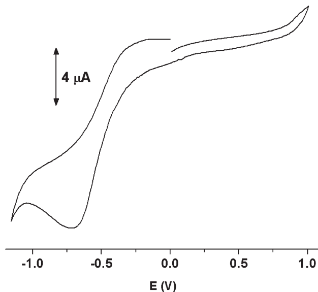
Fig. 3 Cyclic voltammogram of the complex in methanol containing TBAP as the supporting electrolyte at a scan rate of 100\text{ mV s}^{-1} .
