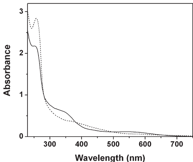
Fig. 2 UV-vis spectra of cobalt(II) chloride with 2-aminomethylpyridine in a 1 : 2 molar ratio in methanol (dashed line) and upon addition of alkaline hydrogen peroxide (solid line).
